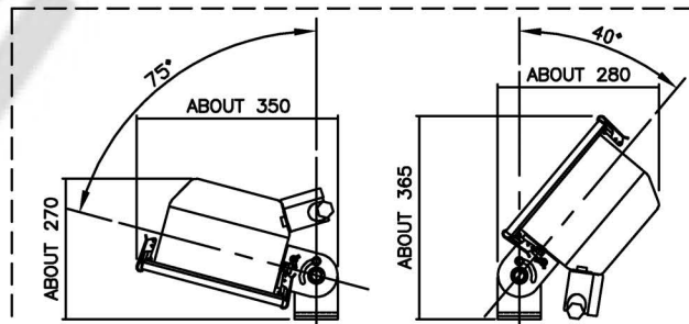
DOWN 75° DIMENSION
