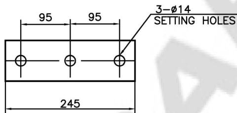
SETTING DIMENSION
